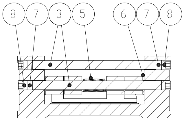
SECTION B-B
